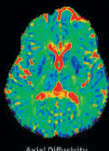
Axial Diffusivity
