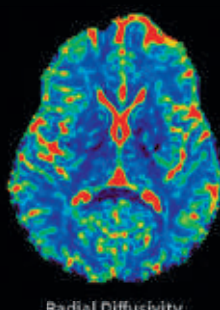
Radial Diffusivity
